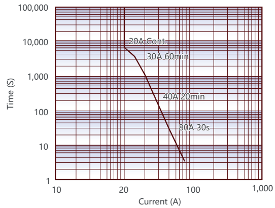
Tolerance curve
