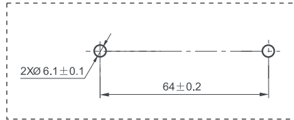
Mounting hole size
